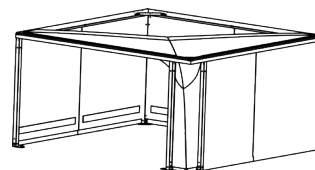
Cyclone
