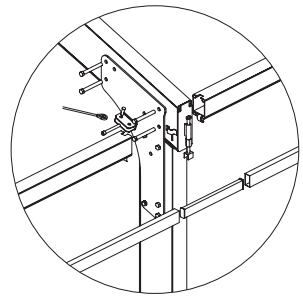
4. eave corner (field)
